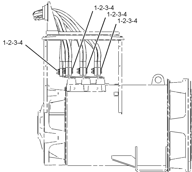
(ALTERNATOR CONNECTION)
