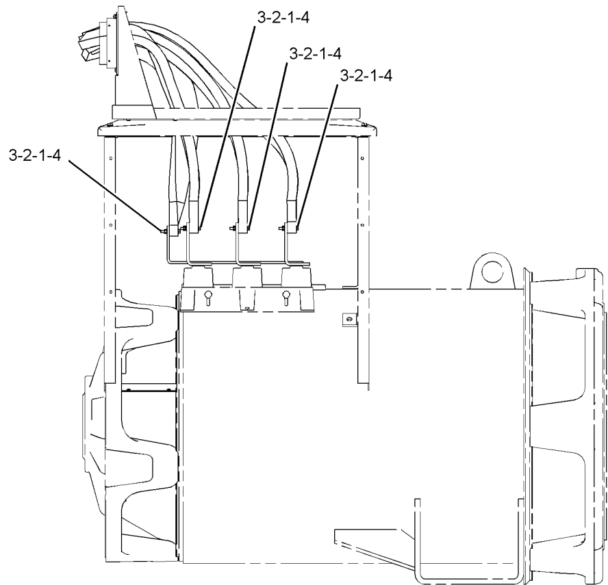
(ALTERNATOR CONNECTION)
