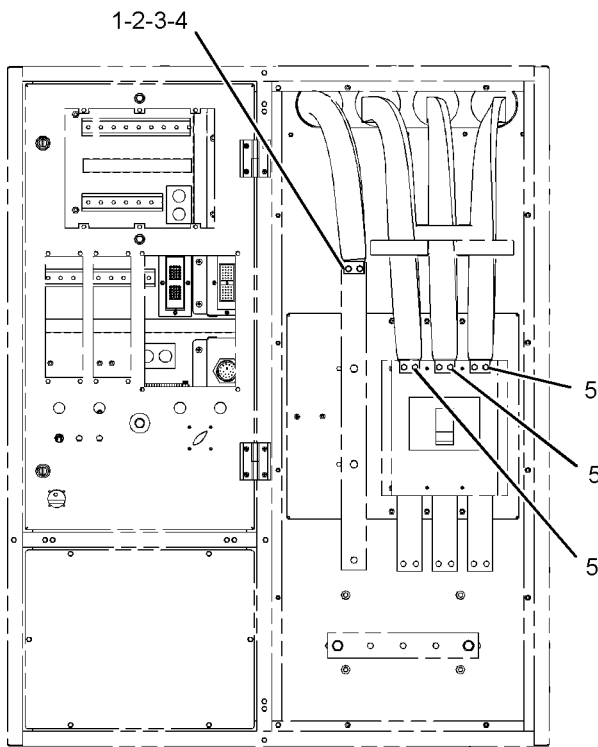
(BREAKER CONNECTION)
