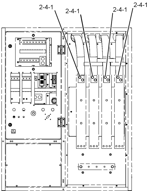
(P.T.S CONNECTION)
