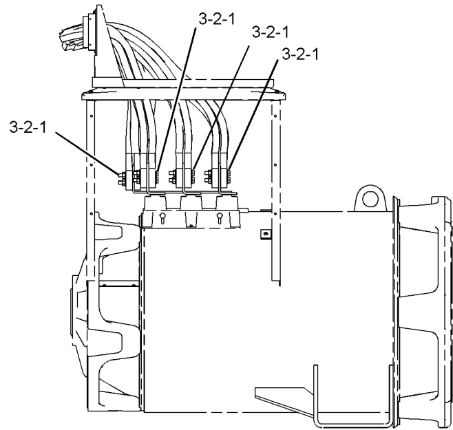
(ALTERNATOR CONNECTION)
