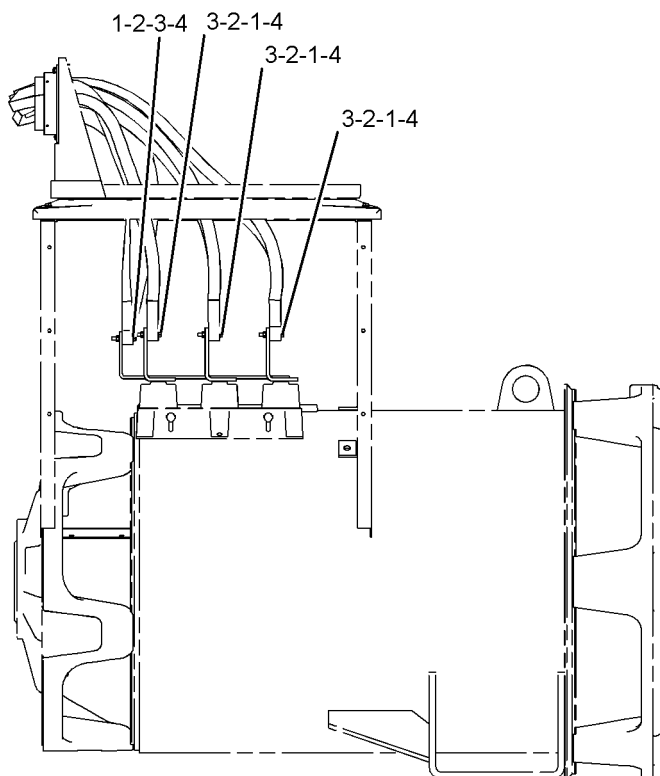
ALTERNATOR CONNECTION <END>
