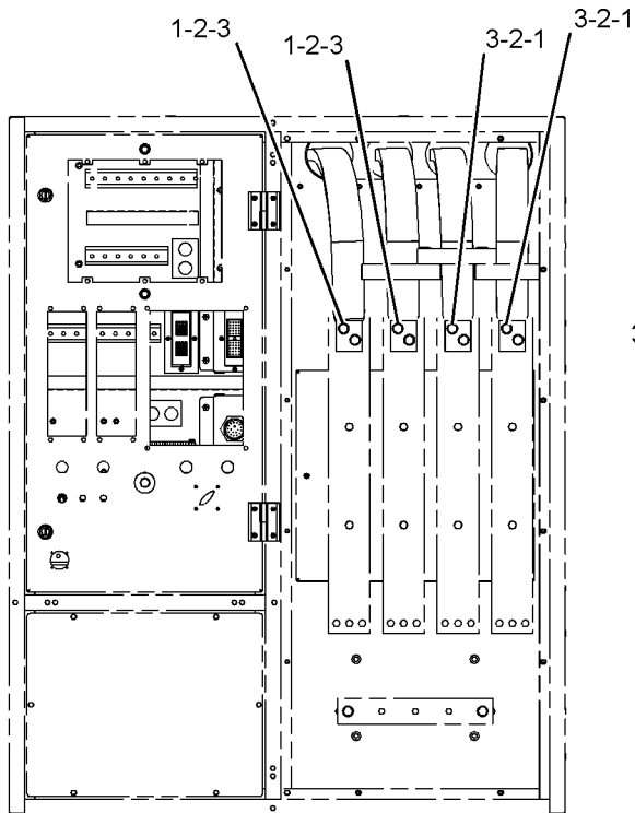
(P.T.S CONNECTION)
