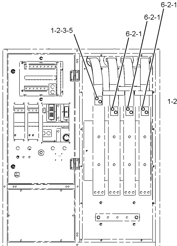
(BREAKER CONNECTION)
