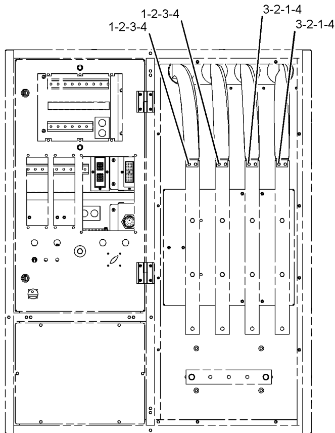
P.T.S CONNECTION
