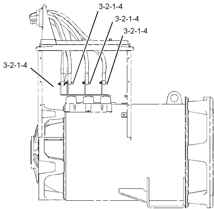
(ALTERNATOR CONNECTION)
